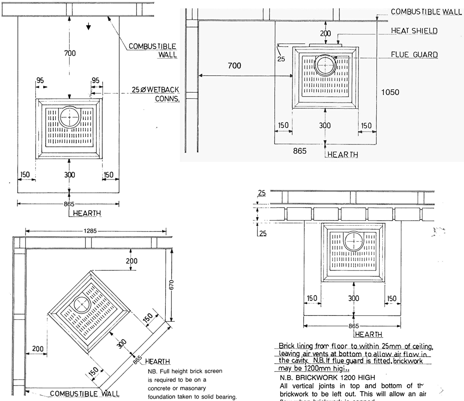
FIG D: HEATER POSITIONS
